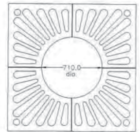
G010 1500 x 1500 x 710 I/D x 25mm Thick Cl:184kg
