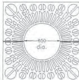
G012B 1400 x 1400 x 650 I/D x 25mm Thick Cl:154kg
