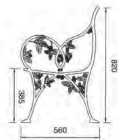
BE006 Front: H385mm Cl:25kg
