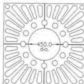
G006 1156 x 1156 x 450 I/D x 25mm Thick Cl:116kg
