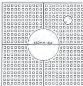
G146 1188 x 1186 x 450 I/D x 25mm Thick Cl:140kg
