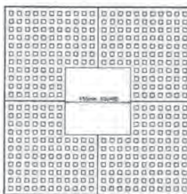
G147 1200 x 1200 x 450 Square Centre x 20mm Thick Cl:140kg
