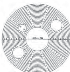
G148 1200 O/D x 400 I/D x 25mm Thick Cl:95kg
