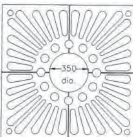
G013A 1220 x 1220 x 350 I/D x 20mm Thick Cl:108kg
