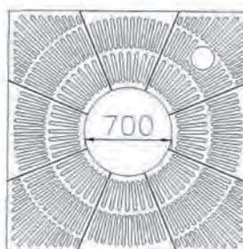
G140 1930 x 1930 x 700 I/D x 25mm Thick Cl:303kg
