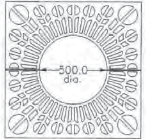
G012 1000 x 1000 x 500 I/D x 25mm Thick Cl:84kg
