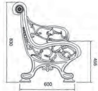
BE003 Front: H455mm Cl:68kg
