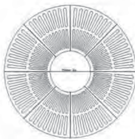
G001 2440 O/D x 750 I/D x 25mm Thick Cl:480kg
