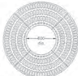
G004A 1525 O/D x 600 I/D x 25mm Thick Cl:124kg
