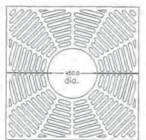
G155 1220 x 1220 x 450 I/D x 25mm Thick Cl:110kg
