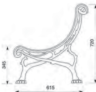
BE004 Front: H345mm Cl:46kg
