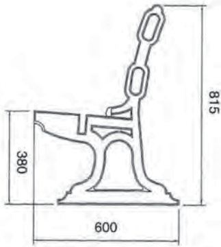
BE007 Front: H380mm Cl:39kg
