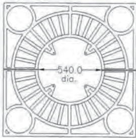
G141B 1125 x 1125 x 540 I/D x 25mm Thick Cl:78kg
