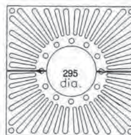
G006A 768 x 768 x 295 I/D x 25mm Thick Cl:45kg
