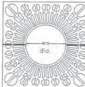
G012C 1750 x 1750 x 815 I/D x 25mm Thick Cl:218kg
