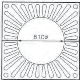
G010A 1000 x 1000 x 610 I/D x 25mm Thick Cl:72kg
