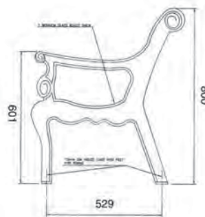
BE019 Front: H601mm Cl:46kg
