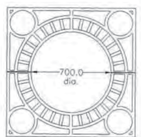
G141A 1125 x 1125 x 700 I/D x 25mm Thick Cl:71kg
