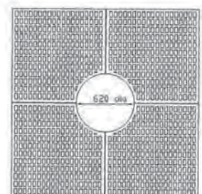
G145 1125 x 1125 x 540 I/D x 25mm Thick Cl:78kg
