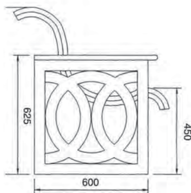
BE013 Front: H450mm Cl:175kg
