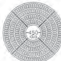
G004B 1800 O/D x 450 I/D x 25mm Thick Cl:190kg
