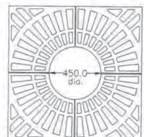
G007 1156 x 1156 x 450 I/D x 25mm Thick Cl:112kg
