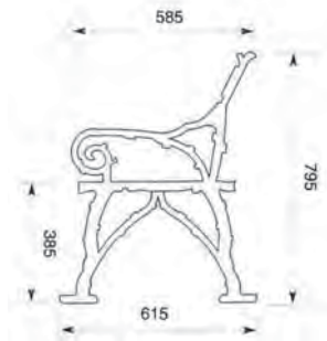
BE017 Front: H385mm Cl:16kg
